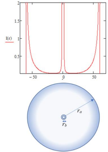
Fig. 1: Graph of the relative elongation function l_r^{(+)}(24) , which determines the relative elongation of a vacuum in the radial direction
