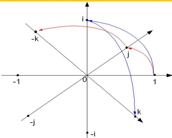
Figure 19, 4D Quaternion rotations compared with Quantum FFF 90 degr. hinging models.
