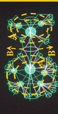
Figure 11, Gravity anomalies by aligned earth internal dark matter black holes.
