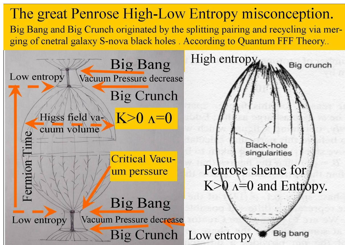
Figure8, The cyclic Multiverse with Entropy development in contrast with Penrose.
