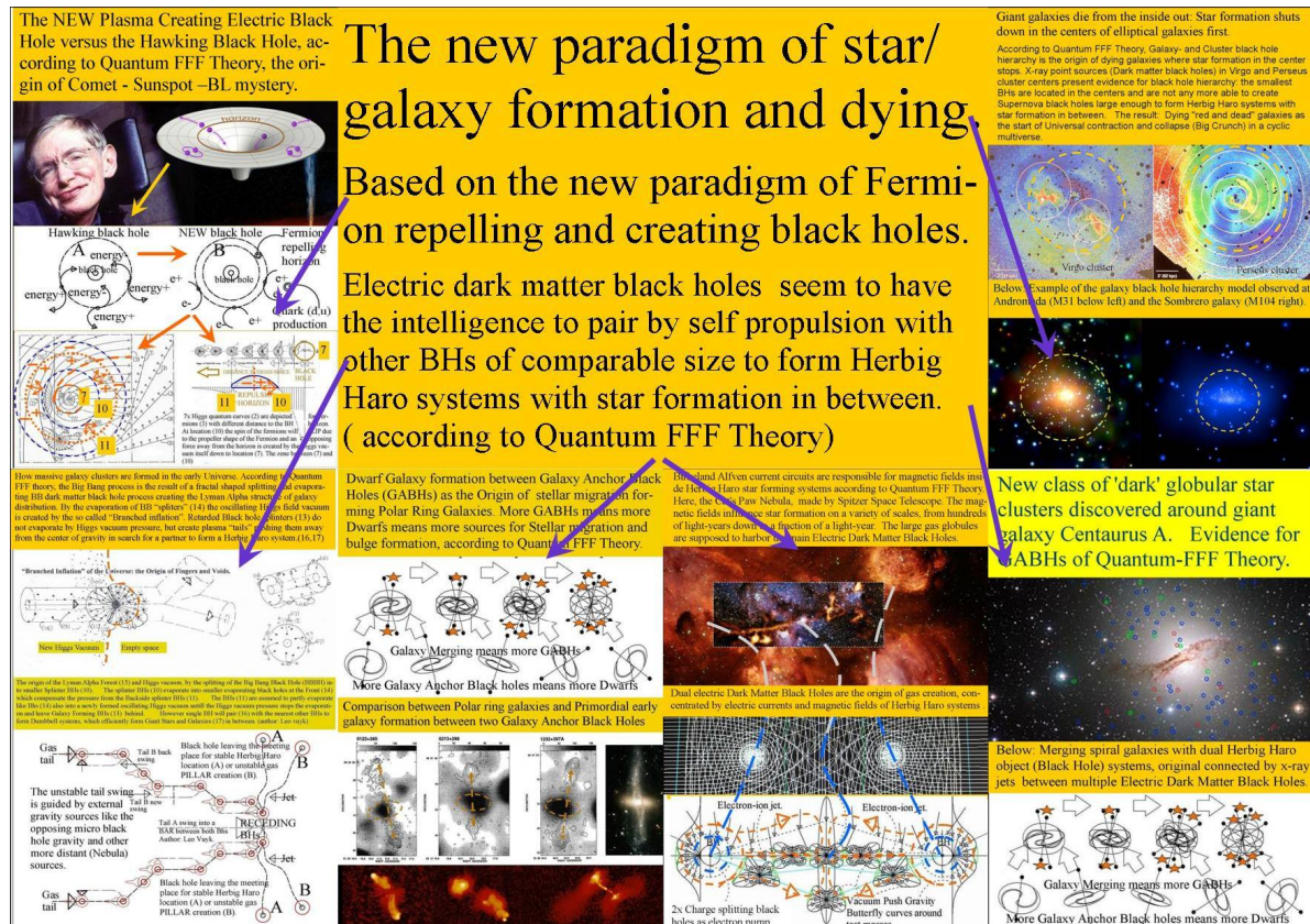
Figure 6, New paradigms according to Quantum FFFTheory.
